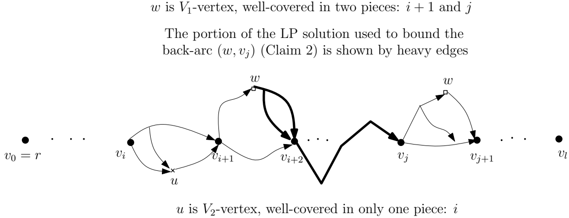
Figure 5.2: Guessed breakpoints v_0, \dots, v_l and flows sent by the LP between consecutive breakpoints.
