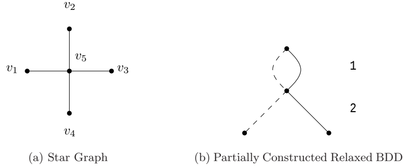
Figure 5.9: A star graph and a partially constructed relaxed BDD for the independent sets in B
