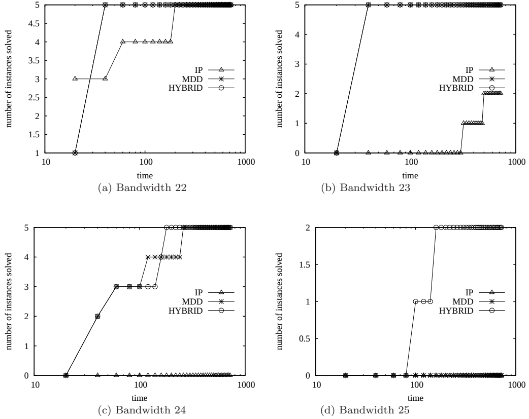
Figure 3.5: Performance profile for pure-IP, pure-MDD, and hybrid MDD/IP for instances width various bandwidth. Time is reported in log-scale.
