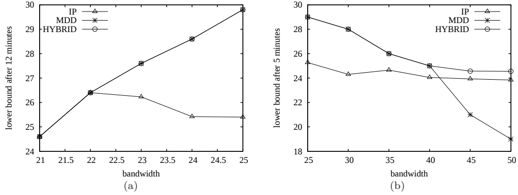
Figure 3.6: (a) Bandwidth versus lower bound (12 minute time limit), (b) Larger bandwidths versus lower bound (5 minute time limit).
