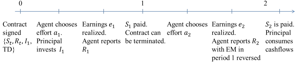
Figure 2.1: Timeline
